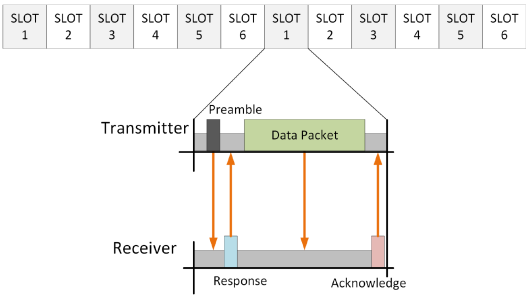
Fig. 8. TSCH: For each timeslot, a determined pair of transmitter and receiver goes online for data transfer.
